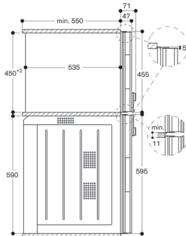
Side view of BM 454/455 above BO
