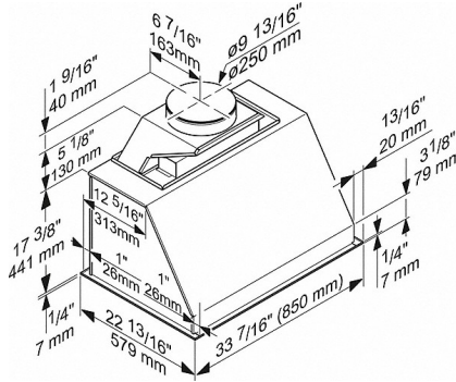
DAR1130 (installation drawing)
