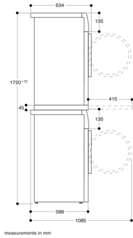
Side view of WT 260 above WM 260 with connection kit accessory
