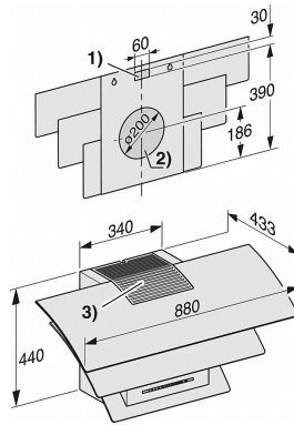
DA 7198 W - Triple (installation drawing)
