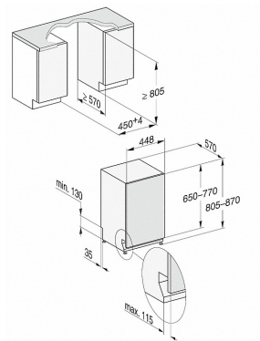
G7000, fully integrated dishwasher, 45cm (installation drawing)
