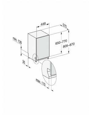
G7000, fully integrated dishwasher, 45cm (installation drawing)
