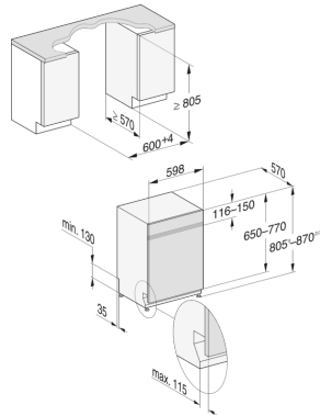
G7000, integrated dishwasher, 60cm (installation drawing)
