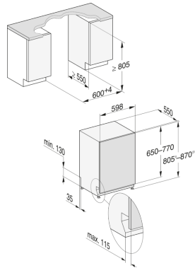
G7000, fully integrated dishwasher, 60cm (installation drawing)
