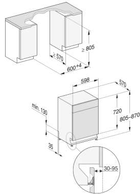
G7000, built under, dishwasher, 60cm (installation drawing)
