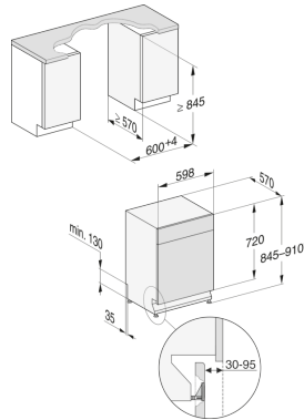
G7000, built under, XXL, dishwasher, 60cm (installation drawing)
