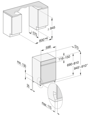
G7000, integrated dishwasher, XXL, 60cm (installation drawing)
