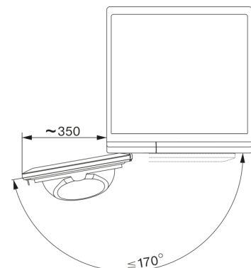
T1 drawing, slanted facia or straight facia, measures in mm
