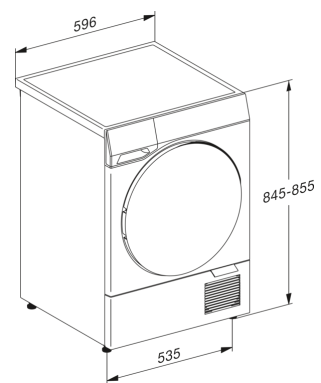
T2 drawing, facia 17 degree, measures in mm
