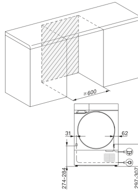
T2 drawing, facia 17 degree, measures in mm
