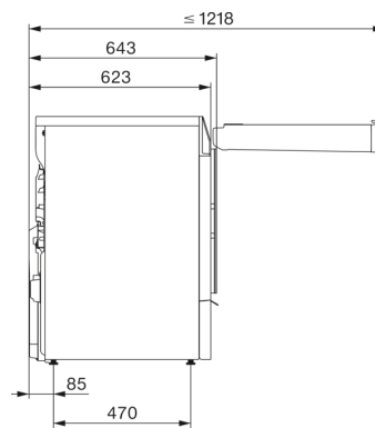
T2 drawing, facia 17 degree, with QuickPowerDry, measures in mm
