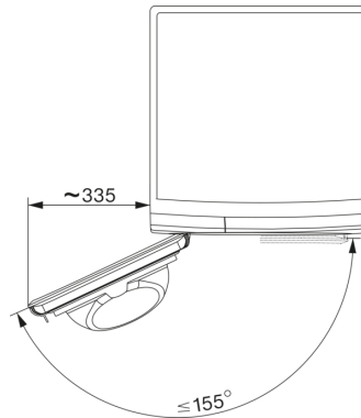
T1 drawing, facia 5 degree, measures in mm
