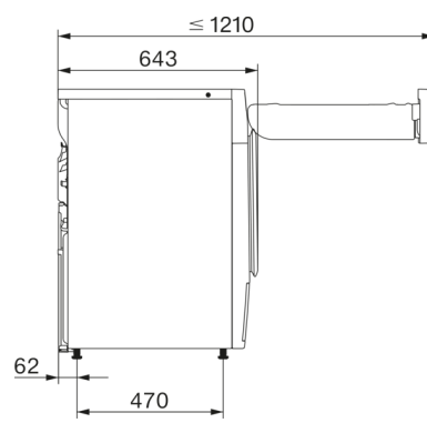
T1 drawing, facia 5 degree, with porthole, measures in mm
