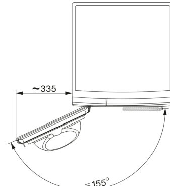
T1 drawing, facia 5 degree, measures in mm
