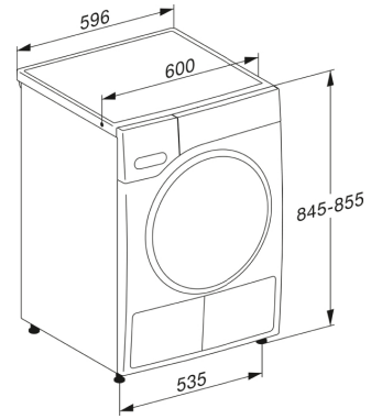
T1 drawing, facia 5 degree, measures in mm
