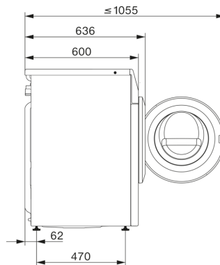
W1 drawing, slanted fascia or straight fascia, measures in mm
