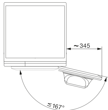
WT1 8/5 kg, drawing, slanted facia or straight facia, measures in mm
