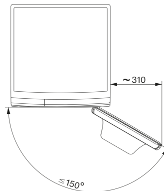
W1 drawing, facia 5 degree, measures in mm
