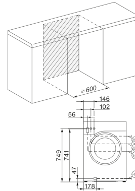
W1 drawing, facia 5 degree, measures in mm
