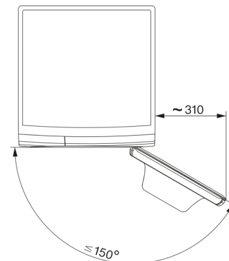
W1 drawing, facia 5 degree, measures in mm
