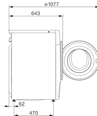
W1 drawing, facia 5 degree, measures in mm
