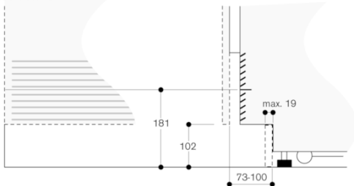
In relation to the standard height of the appliance, the height of the toe kick plate is 102 mm. Maximum thickness of the toe kick plate is 19 mm.
