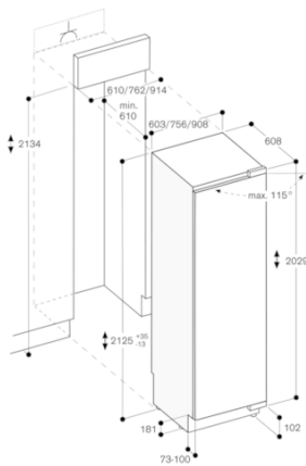
The maximum door front dimensions are designed for a clearance of 3 mm.
