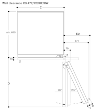
The drawing is based on a furniture front thickness of 19 mm as well as the height of a Gaggenau furniture handle of 49 mm.
