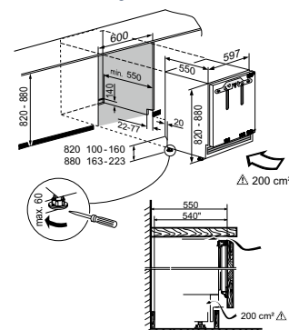
Ventilation Diagram
