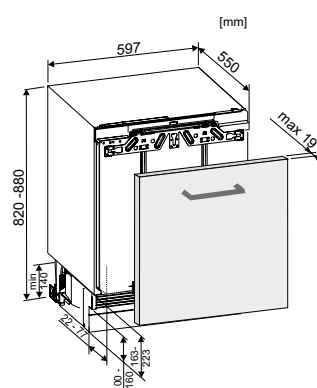
Installation Diagram
