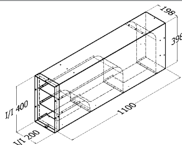
308. BD/WV/K-H-3 Kit assembled as one piece. Three Single Motor Back Draft Wall Vent Horizontal with telescopic length & cover.
