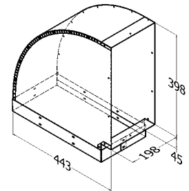
309. VB-3 Vertical Bend Triple Motor 90°
