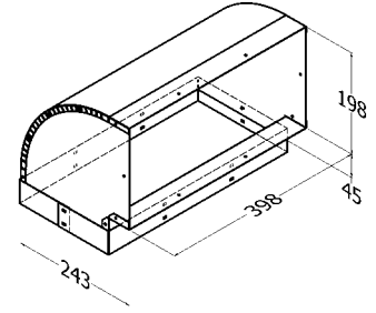
303. HB-3 Horizontal Bend Triple Motor 90°
