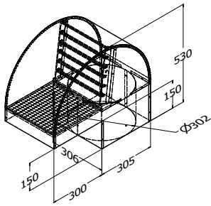
228. BD/SQ-RC 300 BD/SQ-RC 300 CP Back Draft Roof Cowl 300ø
