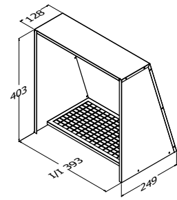
230. WVC-300 WVC-300 SS Wall vent cover to suit single motor 300ø
