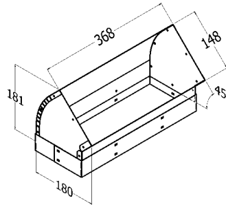
205. HB-2/45 Horizontal Bend Twin Motor 45°
