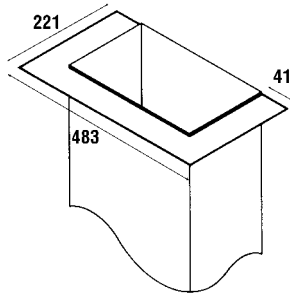
252. CF 3F-1200-2 Ceiling Flange to suit 3F 1200-2
