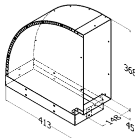
211. VB-2 Vertical Bend Twin Motor 90°
