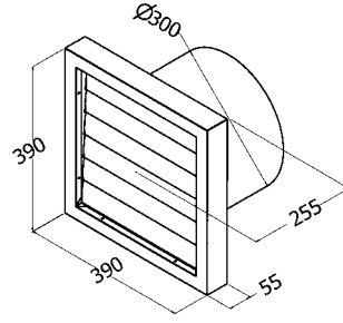
229. BD/WV-300 Back Draft Wall Vent 300ø
