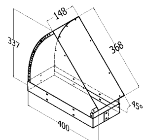
212. VB-2/45 Vertical Bend Twin Motor 45°
