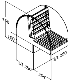
243. BD/RC-250 SQ BD/RC-250 SQ CP Wall Vent Cover 250SQ
