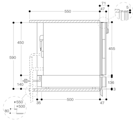
Side view WS 461 under BS, BM, CM
