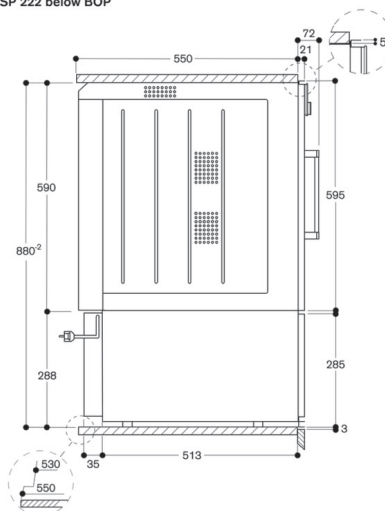
WSP 222 below BOP
